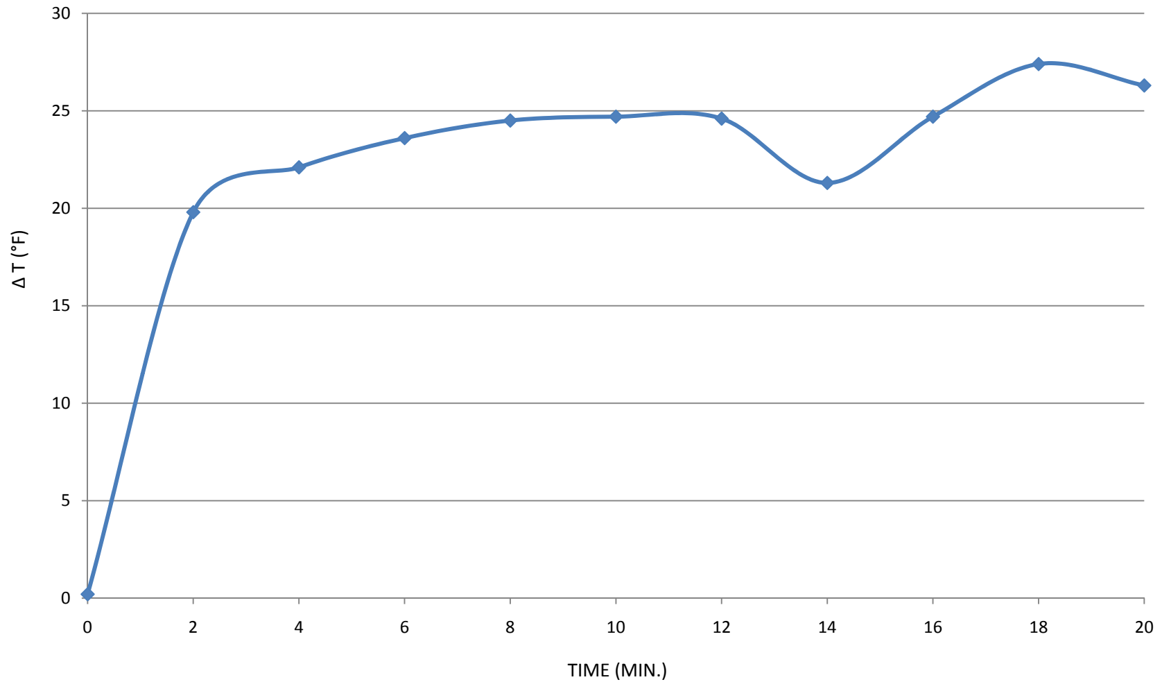
Temperature Drop vs. Time (Post Turning Evaporative Cooling Unit On)
